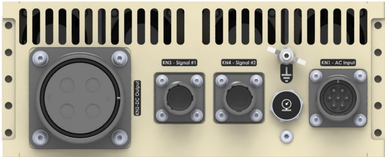
Figure 18. Connector Panel
