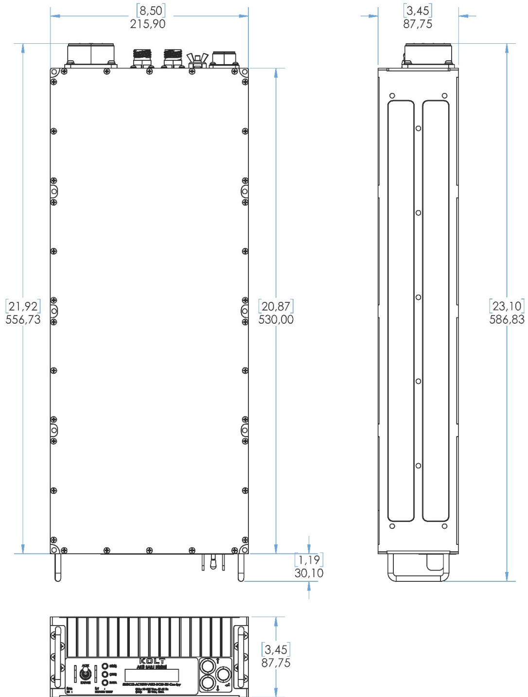
Figure 28. Mechanical Dimensions
