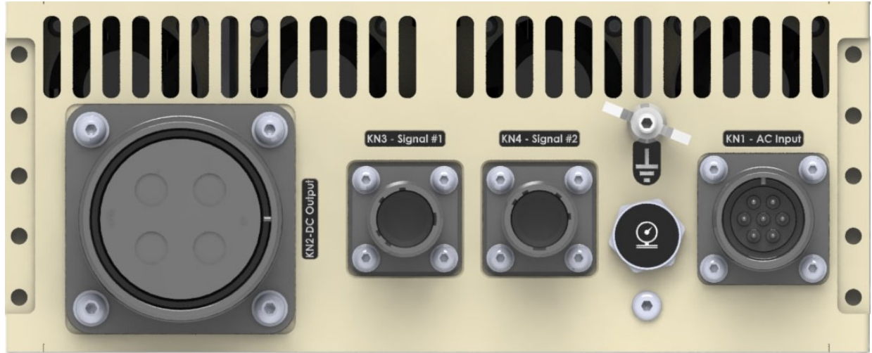
Figure 18. Connector Panel
