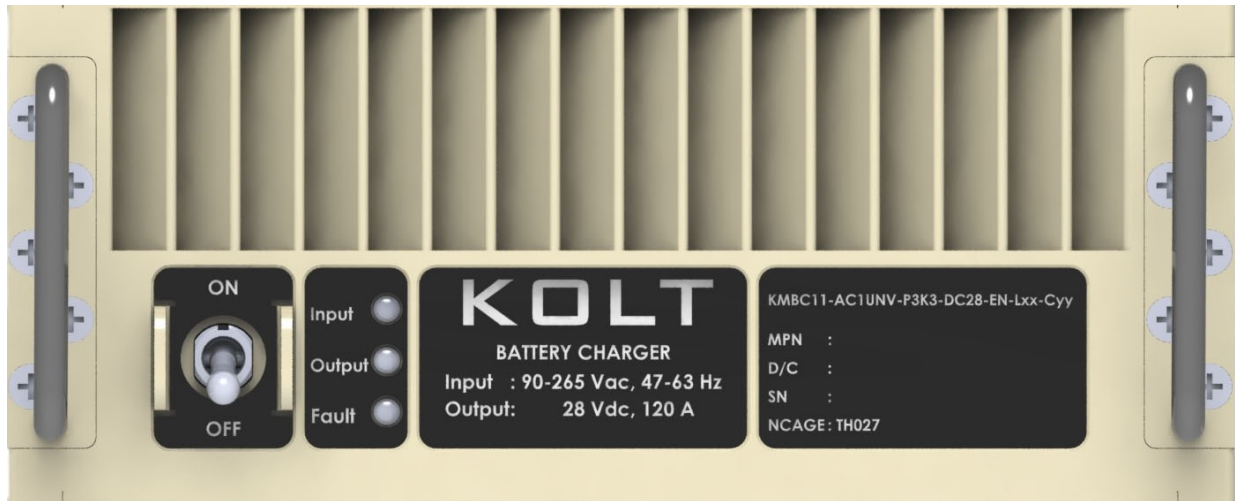
Figure 23. Front Panel
