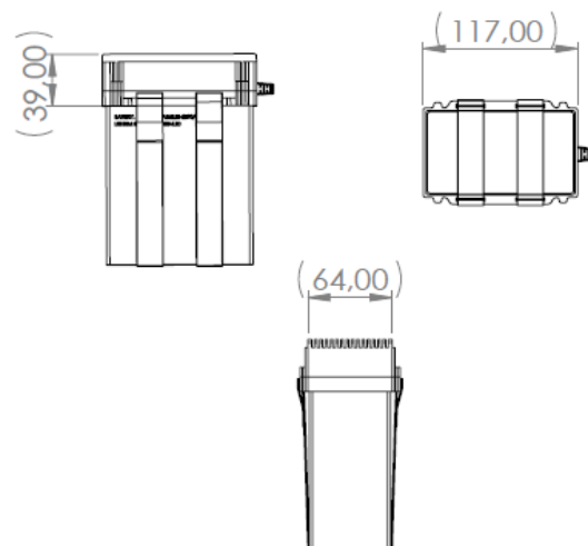
Outline Drawing(mm)
